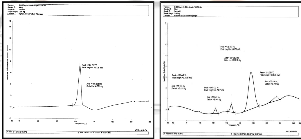
Fig. 6: DSC of pure rosiglitazone maleate
