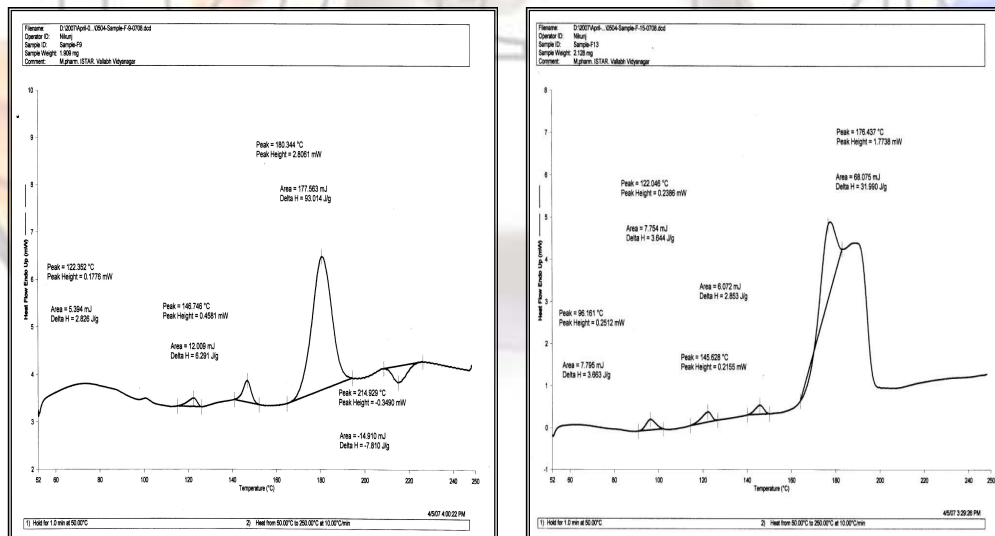
Fig. 8: DSC of physical mixture of rosiglitazone maleate with CP-934 and NaCMC
